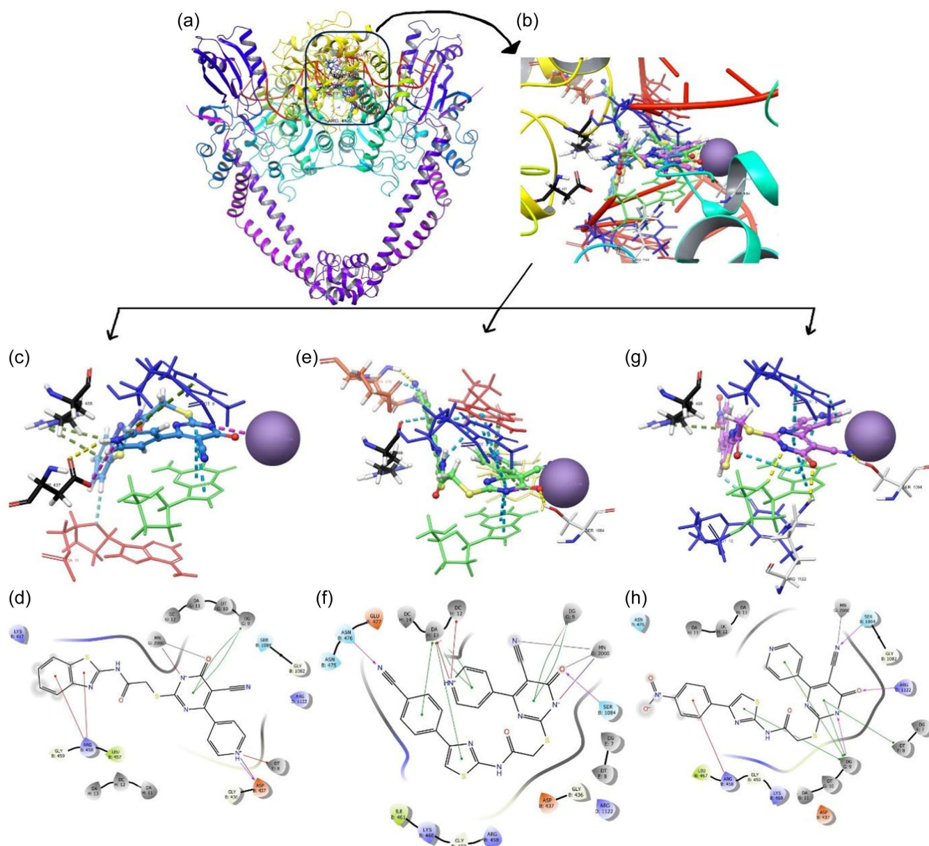
FIGURE 3 Interaction of active compounds with DNA and DNA gyrase and molecular docking results. (a) Image of the active site with DNA and DNA gyrase. (b) Zoomed three-dimensional (3D) image of active inhibitors superimposed in the enzyme active site. (c) and (d) 3D and two-dimensional (2D) pose for compound 5a ; (e) and (f) 3D and 2D pose for compound 6b ; (g) and (h) 3D and 2D pose for compound 6c .
